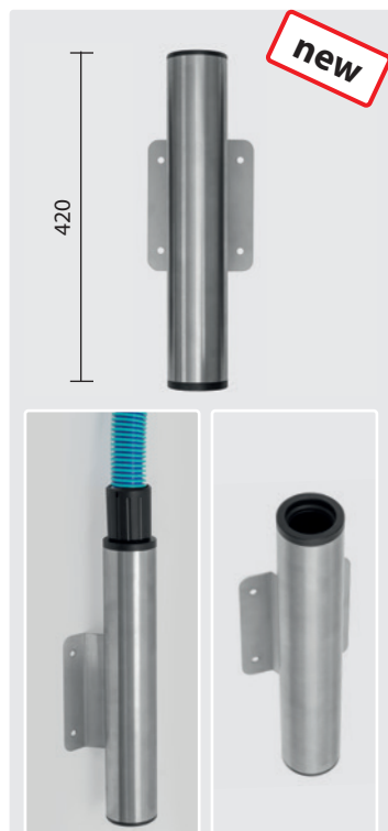
Crevice nozzle holder for wall mounting. Stainless steel
