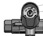
A - Hexagon nut B - Setting marking
