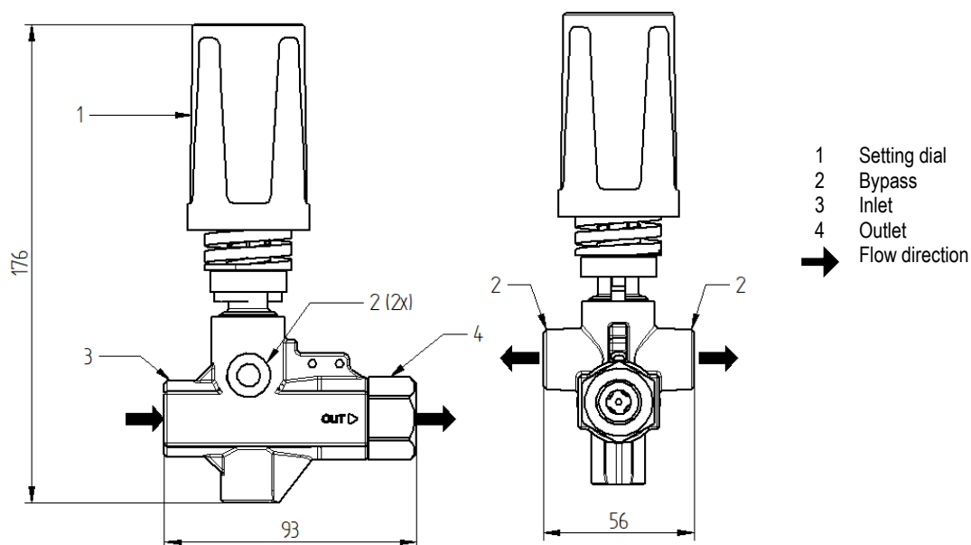
Fig. shows standard variant
